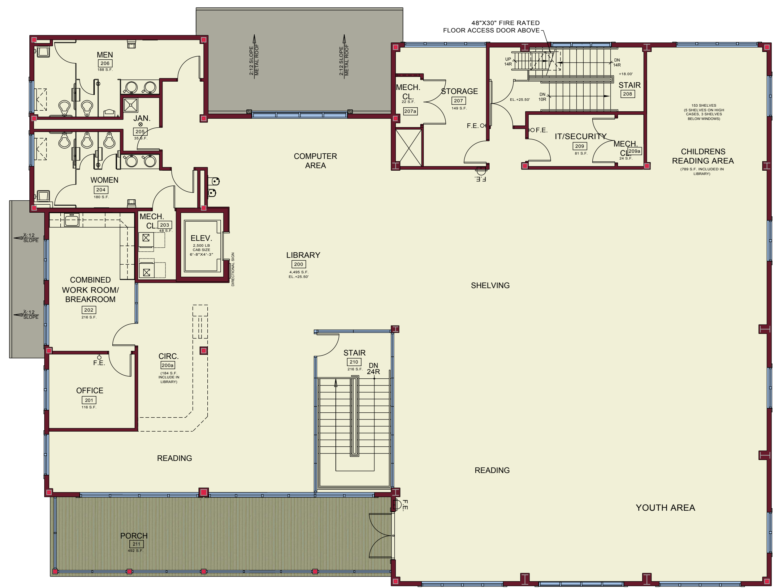
SECOND FLOOR PLAN 6,448 SQ.FT. (EXCLUDE DECK) 1ST FLOOR: 6,790 S.F. 2ND FLOOR: GROSS AREA 6,448 S.F. MECH. ATTIC: GROSS AREA 333 S.F. TOTAL FLOOR: 13,571 S.F.
