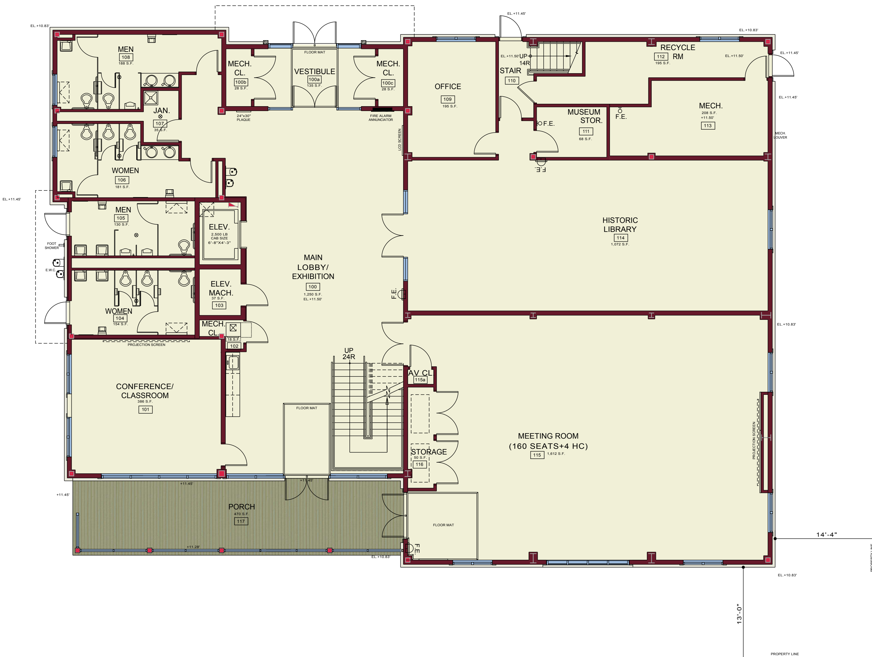
10' BULKHEAD SETBACK FIRST FLOOR PLAN 6,790 SQ.FT. (EXCLUDE DECK)
